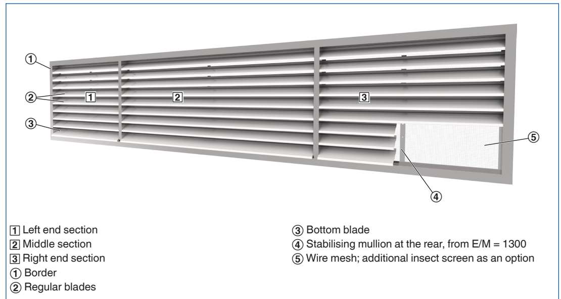
Schematic illustration of WL-B-AL
