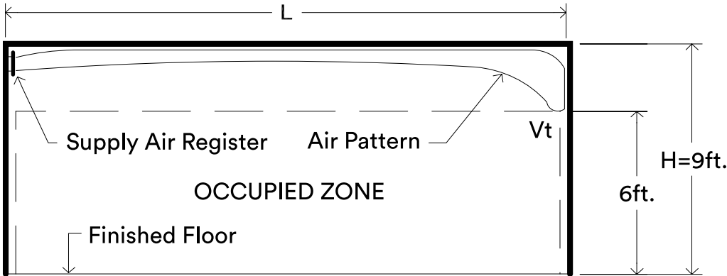
ELEVATION VIEW
